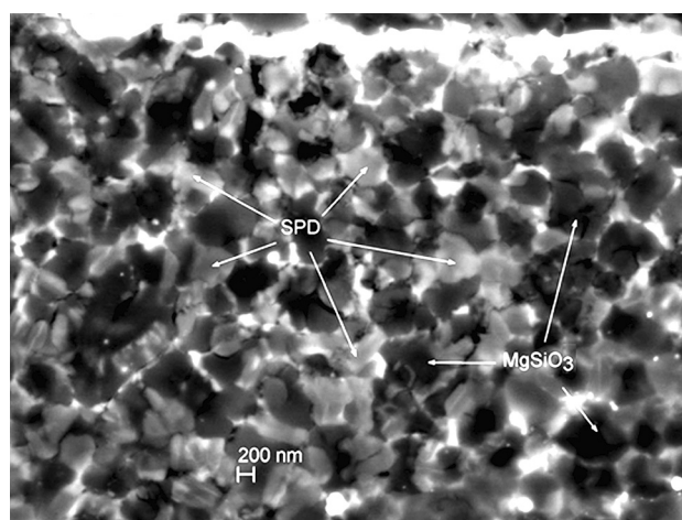
Fig. 25 BSE image showing the fine-grained partly inverted ringwoodite (\text{Mg,Fe,Si})_2(\text{Si},\square)\text{O}_4 with (\text{Mg,Fe})\text{SiO}_3 within the matrix of a melt vein in Ol olivine, Rwd ringwoodite, FeNi FeNi metaSuizhou meteorite (after Ma et al. 2019b)
