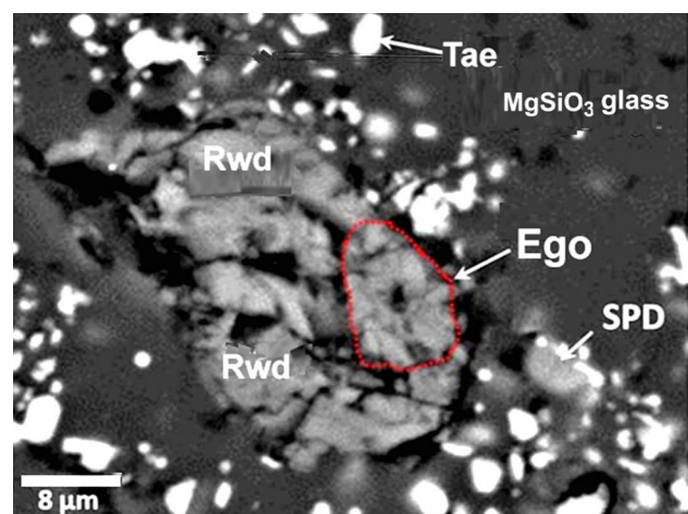
Fig. 5 BSE image showing the occurrence of elgoresyite ( Ego ), indicated with the dotted red line, which is associated with ringwoodite ( Rwd ) and a spineloid silicate ( SPD ; Ma et al 2019b) within \text{MgSiO}_3 glass (after Bindi et al. 2021)
