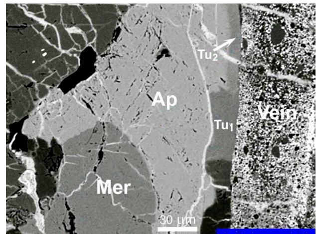
Fig. 17 BSE image showing a composite phosphate grain directly adjacent to the left wall of a Suizhou shock melt vein. Note the dark gray tuite ( Tu 1 ) formed from merrillite ( Mer ), and the gray band of tuite ( Tu 2 ) formed from decomposition of chlorapatite ( Ap ). White lines penetrating minerals and shock vein are injected FeS veinlets (after Xie et al. 2016a)
