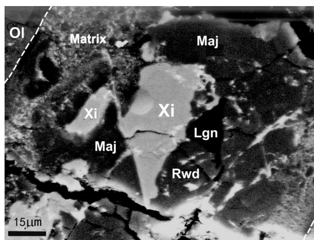
Fig. 20 BSE image showing two xieite ( Xi ) grains surrounded by other high-pressure minerals ringwoodite ( Rwd ), majorite ( Maj ), and lingunite ( Lgn ) in a Suizhou shock melt vein (after Xie and Chen 2016)
