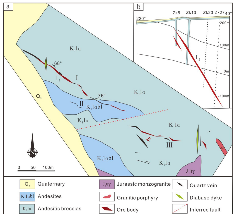
Fig. 3 a Geological map of the Sandaowanzi ore deposit and b Cross-section of the I 2 orebody (revised after Lü 2011)
