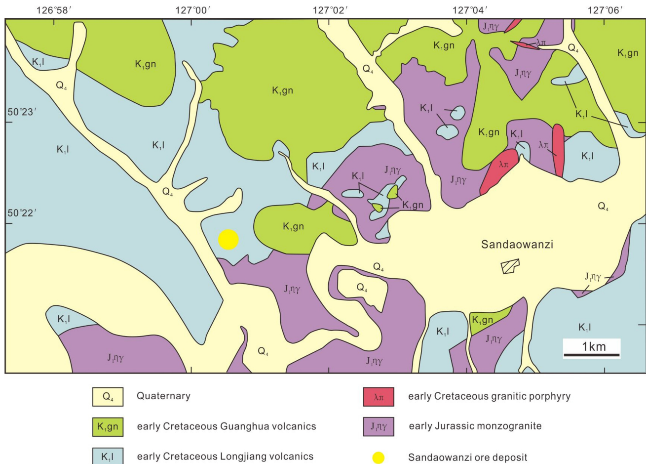
Fig. 2 Geological map of the Sandaowanzi area (revised after Wang et al. 2017)
