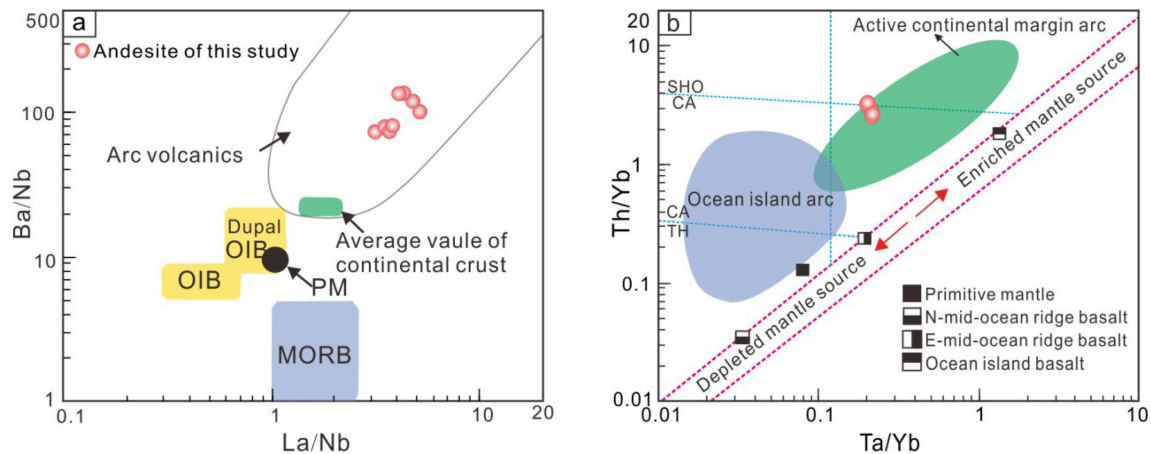
Fig. 12 a Ba/Nb versus La/Nb classification diagram (after Jahn et al. 1999); b Ta/Yb versus Th/Yb (after Pearce 2008) tectonic discrimination diagrams for the andesites of Longjiang Formation in Sandaowanzi gold deposit
