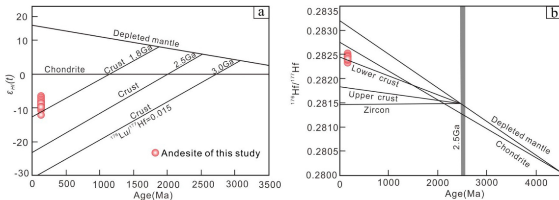
Fig. 8 Zircon Hf isotopic features for the andesites of Longjiang Formation in Sandaowanzi gold deposit (after Yang et al. 2006)
