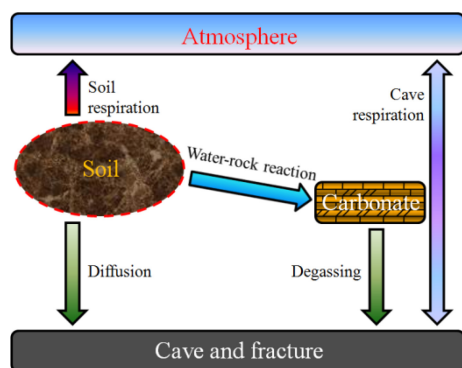
Fig. 12 Conceptual model of soil air CO 2 emissions in the KCZ. The water–rock reaction and degassing are positive and negative reactions of \text{CO}_2 + \text{H}_2\text{O} + \text{M}(\text{Ca or CaMg})\text{CO}_3 \rightleftharpoons \text{M}^{2+} + 2\text{HCO}_3^- , respectively.
