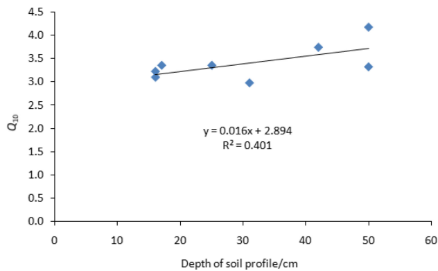
Fig. 10 Relationship between soil depth and Q_{10} among the eight monitoring sites
