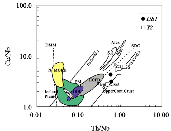
Fig. 13 Ce/Nb-Th/Nb diagram for Carboniferous volcanic rocks from Wulungu-Luliang area (after Song et al. 2004). DMM depleted mantle, SDC recycled subduction-derived component, S.S. subducting sediments in arcs, RSC recycled residual slab composition, OIB ocean-island basalt, N-MORB normal mid-ocean ridge basalt, E-MORB enriched MORB, PM primitive mantle
